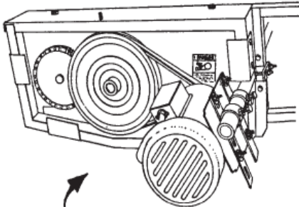
Partially Assembled Safety Shield
