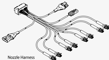
Nozzle Harness 45-04005-08-20
