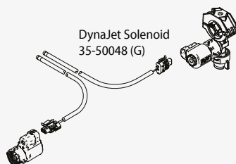
Extension Cables 45-04006-03 45-04006-07 45-04006-13 45-04006-20
